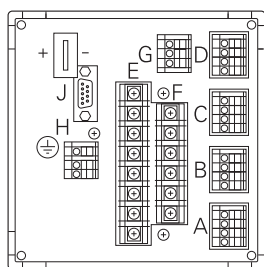
SIMEAS P660
